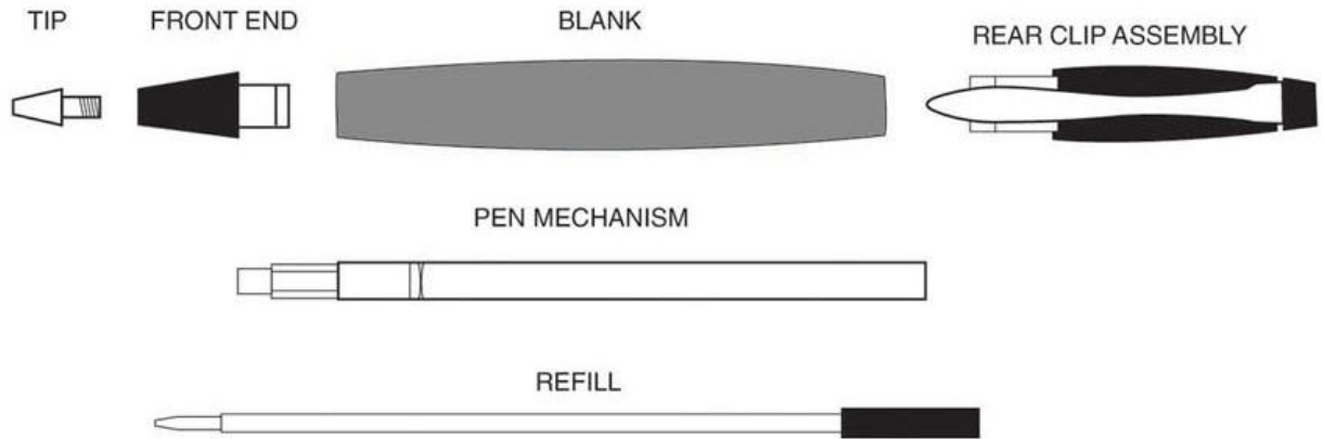
DIAGRAM C - PEN ASSEMBLY
