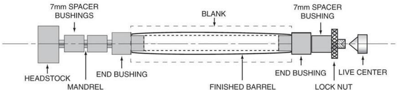
DIAGRAM B - MOUNTING ON THE LATHE
