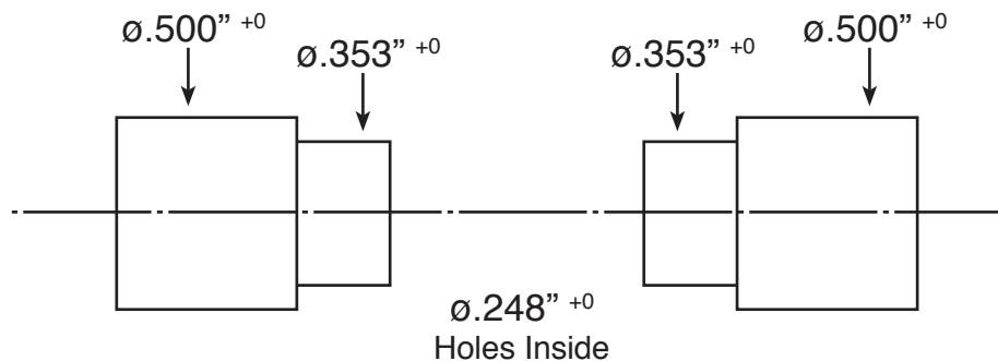
DIAGRAM C • Bushings #6109
