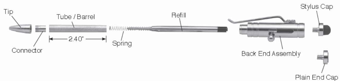
DIAGRAM A / PARTS LAYOUT
